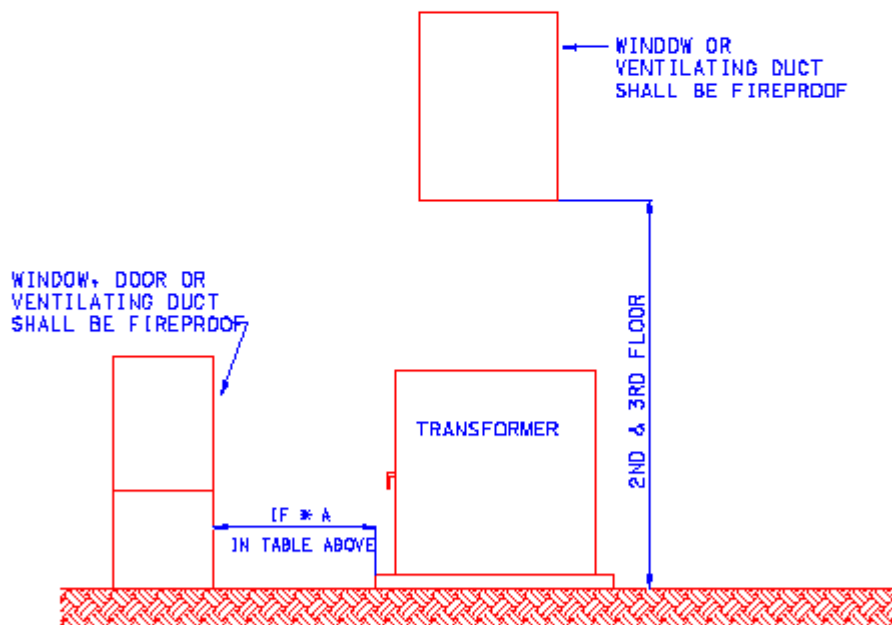
ELEVATION VIEW
