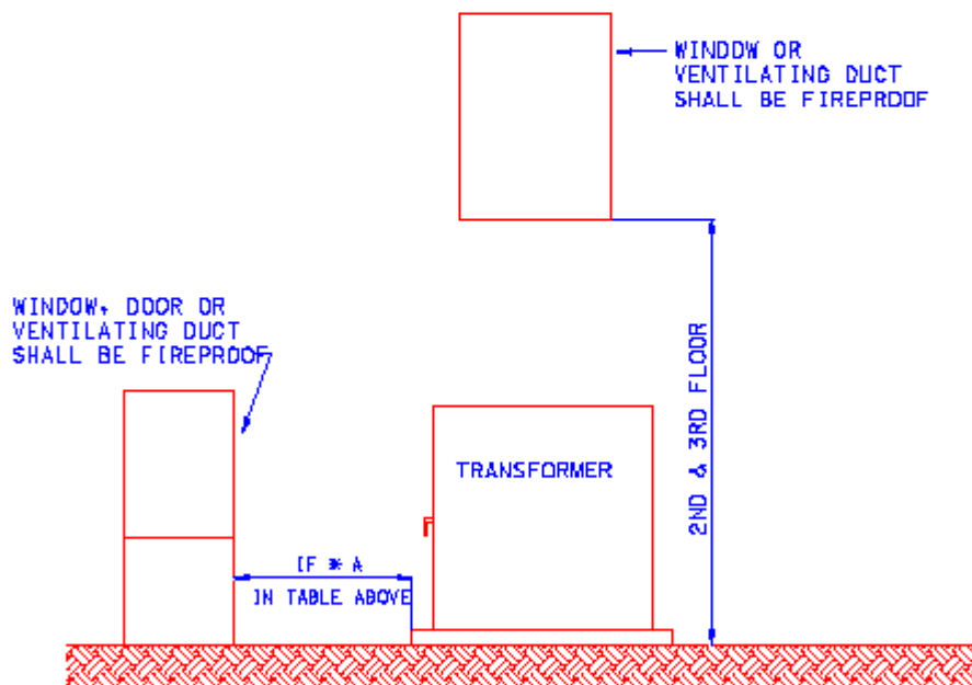
ELEVATION VIEW
