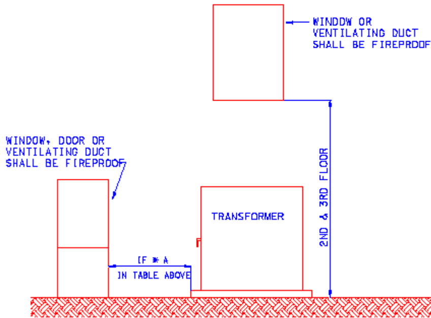
ELEVATION VIEW
